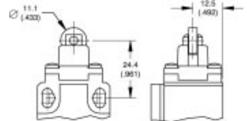
Top Push, Roller Plunger Model No.: PLS-M-TRP
