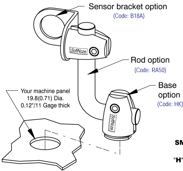
Sensor Mounting System Universal Kits
