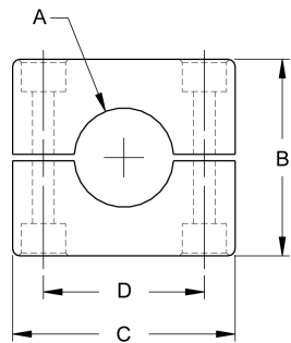
BMS-B Mounting Block only
