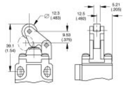
Top Push, Roller Lever Model No.: PLS-M-TRL
