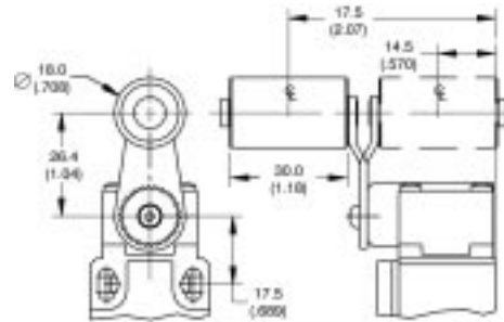
Side Rotary, Wide Roller Lever Model No.: PLS-M-SRLW
