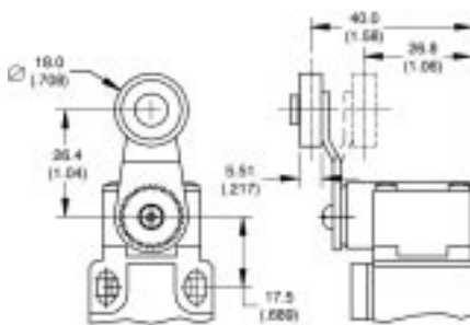
Side Rotary, Roller Lever Model No.: PLS-M-SRL
