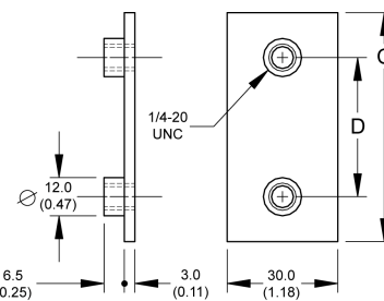
BMS4 - Weld-on Plate
