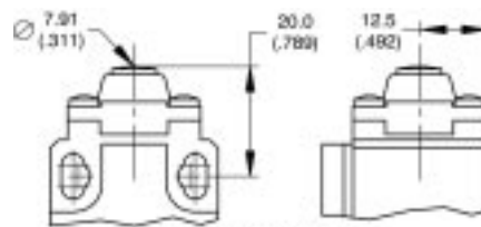
Top Push, Metal Plunger Model No.: PLS-M-TMP
