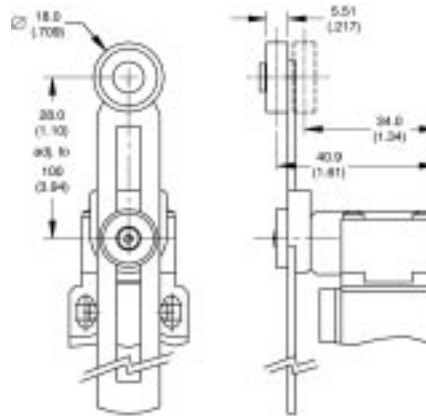
Side Rotary, Adjustable Roller Lever Model No.: PLS-M-SARL
