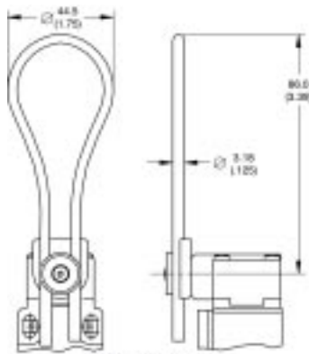
Side Rotary, Plastic Loop Model No.: PLS-M-SR-PL
