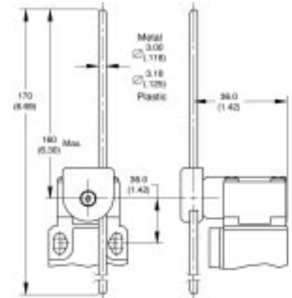
Side Rotary, Metal Rod (Two Models) Model No.: PLS-M-SR-MR Side Rotary, Plastic Rod Model No.: PLS-M-SR-PR
