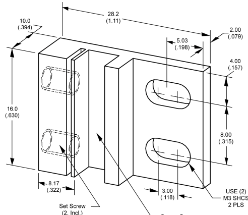
Block Mount Micro-type 1
